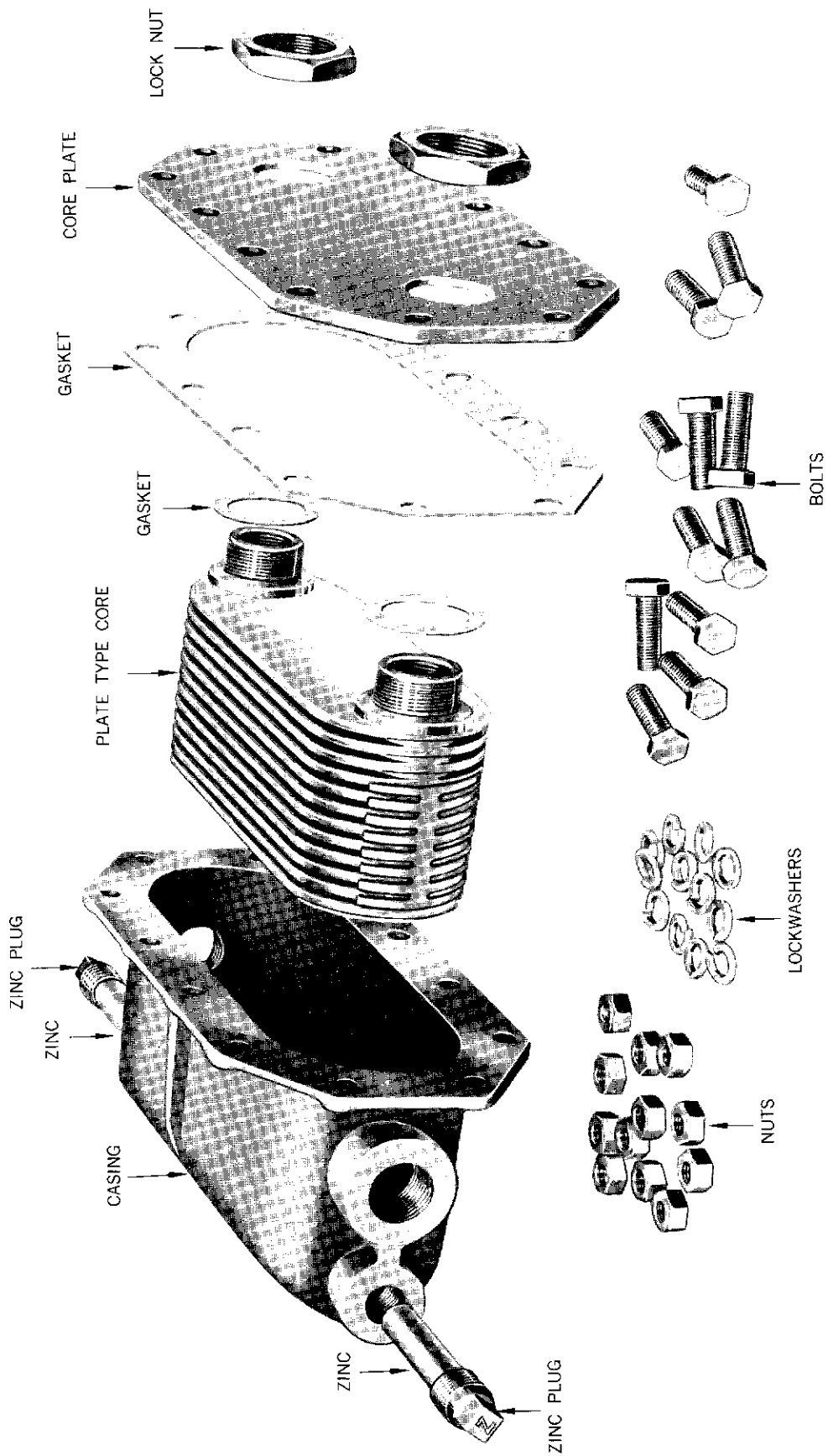
EXPLODED VIEW OF BASIC MODEL HE 1250
