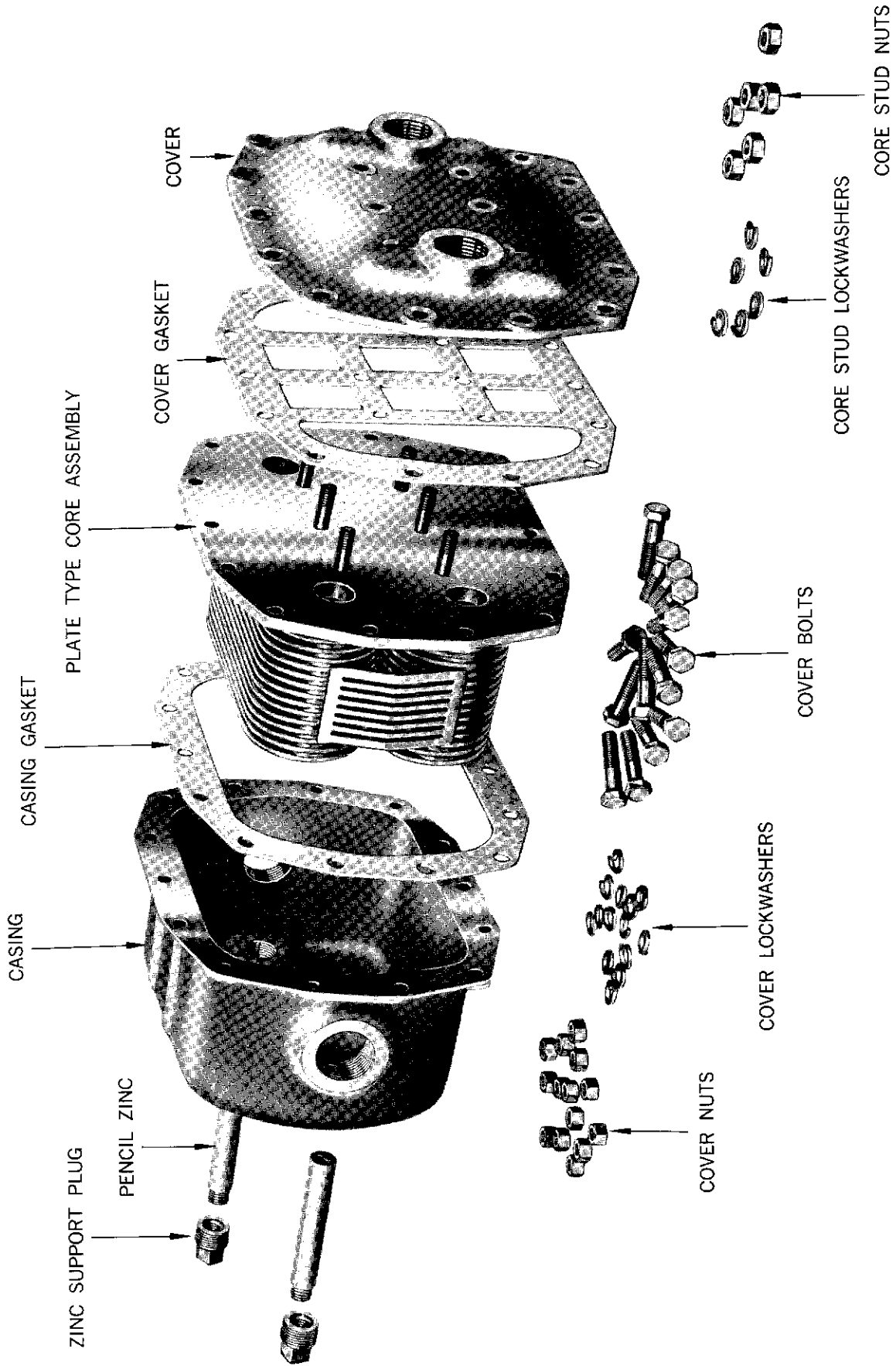
EXPLODED VIEW OF BASIC MODEL HE 1060
